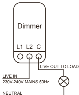
1 Way Dimming
