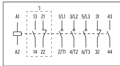
*1 - Optional auxiliary contact unit
