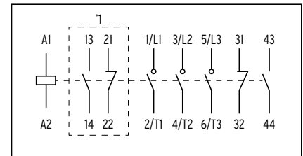
*1 - Optional auxiliary contact unit
