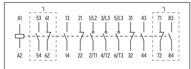
*1 - Optional auxiliary contact unit
