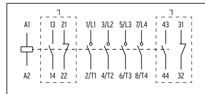
*1 - Optional auxiliary contact unit
