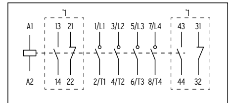
*1 - Optional auxiliary contact unit
