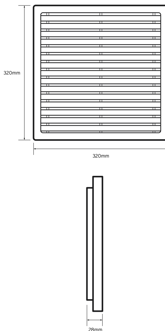
Technical Drawing
