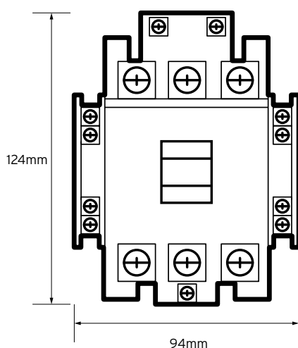
Technical Drawing
