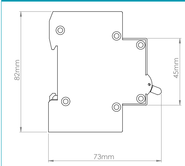
Technical Drawing 4 Pole
